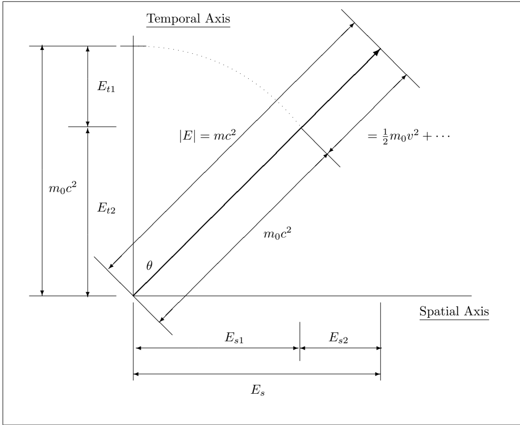
Fig. 3.1 Spatial - Temporal Distribution of Matter Energy.
