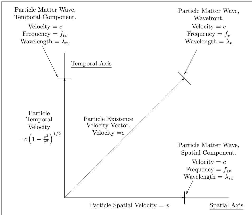
Fig. 2.1 Pictorial Representation of the Matter Wave Associated with a Particle in D_0
